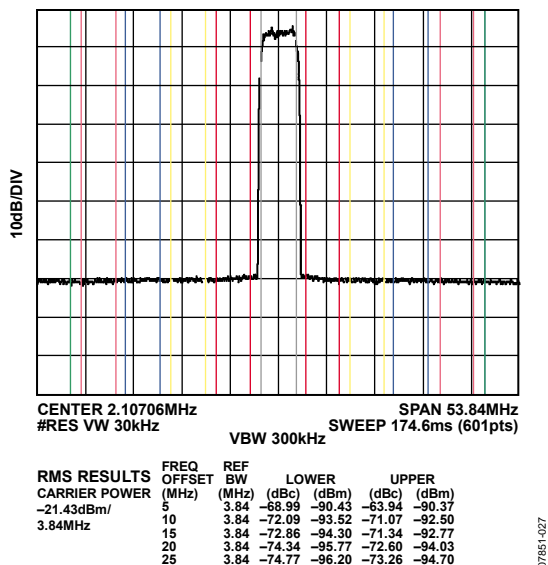
Figure 27. Typical Single-Carrier WCDMA ACLR Performance at 2.1 GHz, f_{DAC} = 2457.6 MSPS (Second Nyquist Zone)
